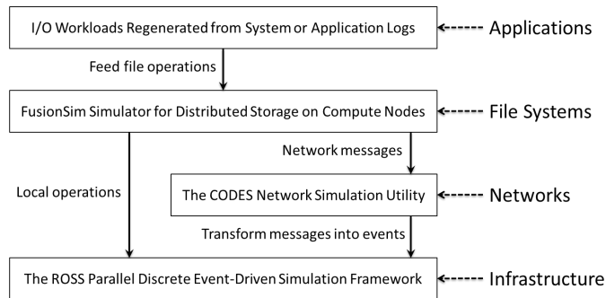
Figure 2. The software stack of FusionSim
