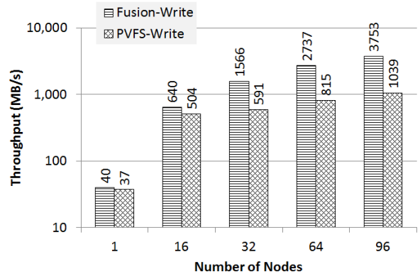
Figure 11. Write throughput on Amazon EC2 Cloud
