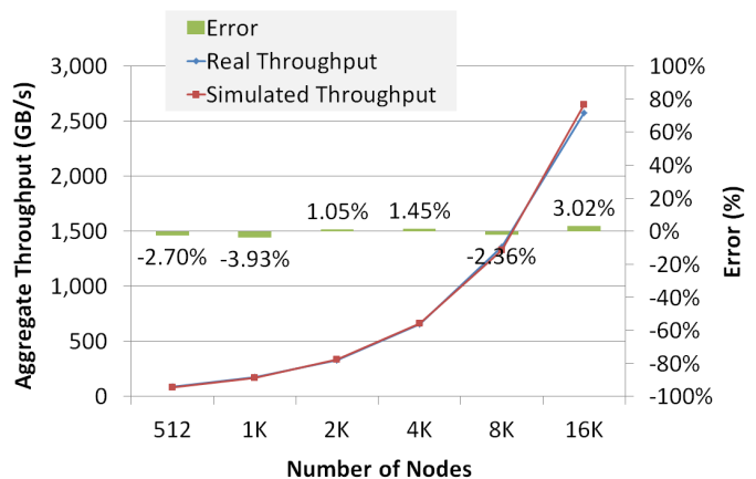
Figure 18. Validation of FusionSim on Intrepid
