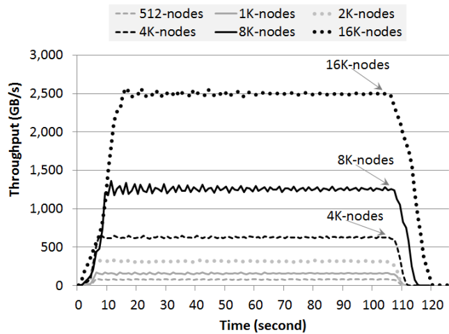
Figure 17. FusionFS scalability on Intrepid
