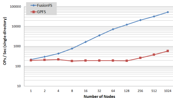
Figure 4. Metadata performance of FusionFS and GPFS on Intrepid (single directory)
