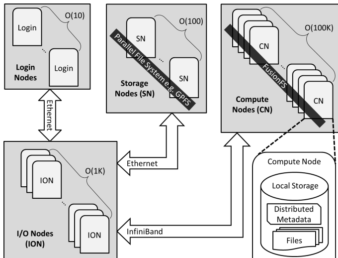
Figure 1. FusionFS deployment in a typical HPC system
