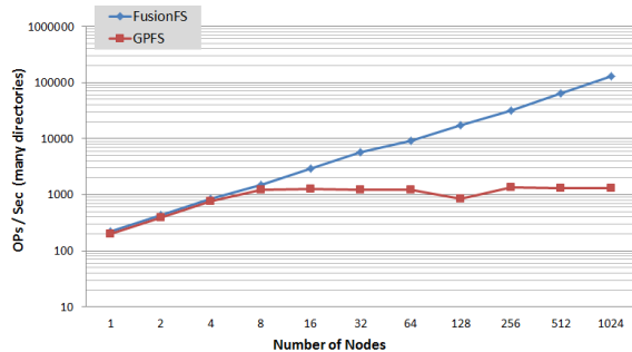
Figure 3. Metadata performance of FusionFS and GPFS on Intrepid (many directories)
