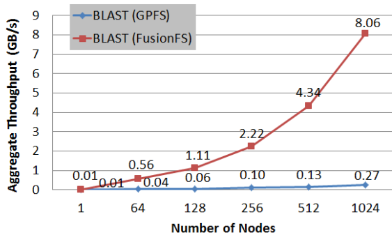
Figure 16. BLAST I/O throughput on Intrepid
