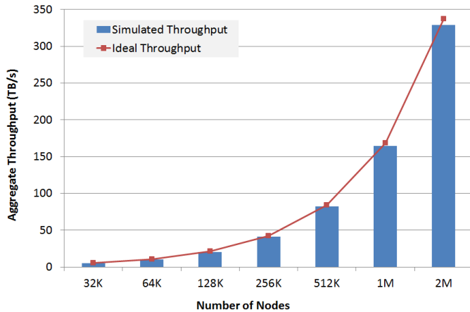
Figure 19. Predicted FusionFS throughput by FusionSim
