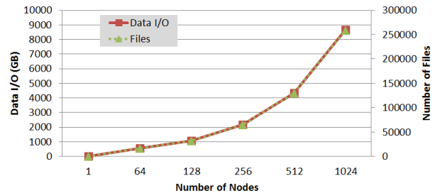
Figure 13. The workload over three stages of BLAST
