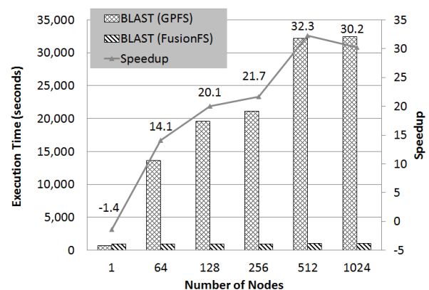
Figure 14. BLAST execution time on Intrepid
