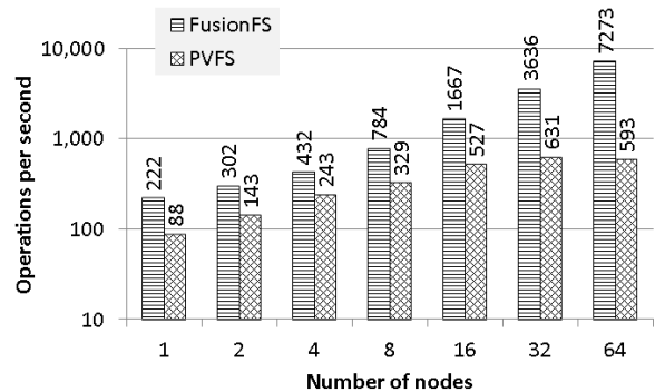
Figure 5. Metadata performance of FusionFS and PVFS on Intrepid (single directory)
