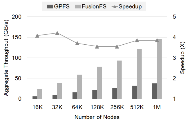
Figure 20. Predicted FusionFS performance with IOR [51], comparing with GPFS
