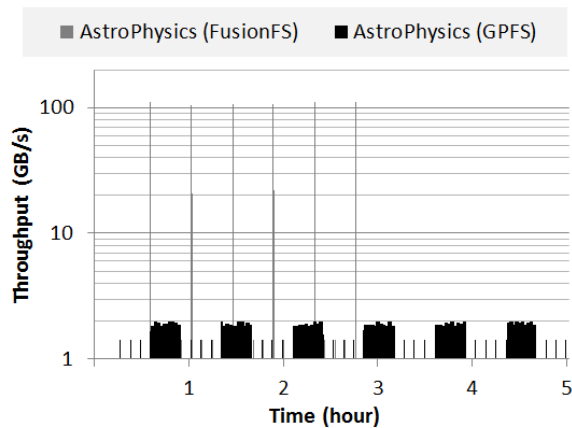
(c) AstroPhysics
