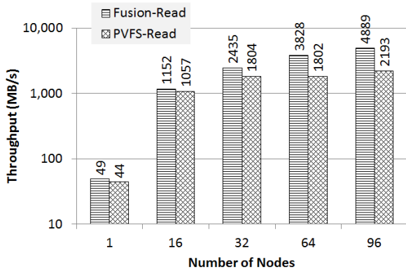
Figure 10. Read throughput on Amazon EC2 Cloud
