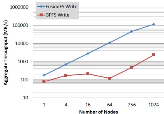
Figure 7. Write throughput of FusionFS and GPFS on Intrepid
