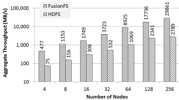
Figure 9. Throughput of FusionFS and HDFS on Kodiak
