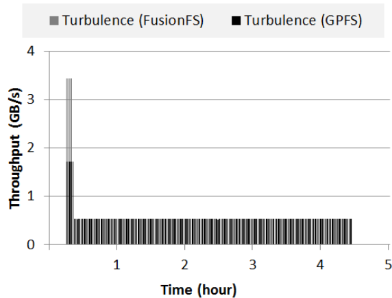
(b) Turbulence
