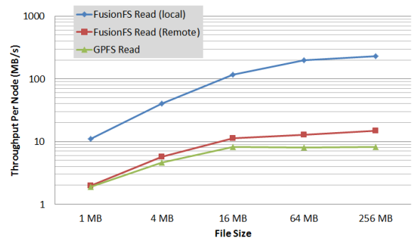
Figure 8. Read throughput of FusionFS and GPFS on Intrepid
