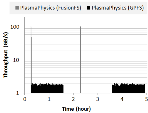
(a) PlasmaPhysics
