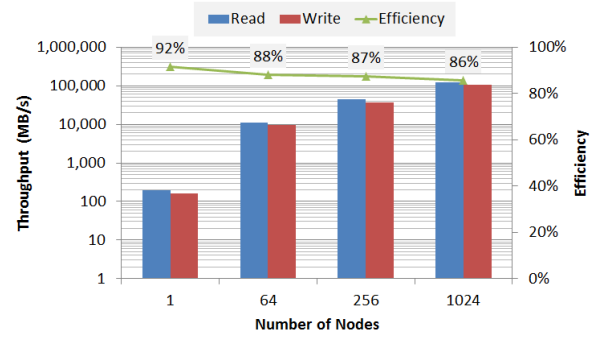
Fig. 15. Throughput on BlueGene/P
